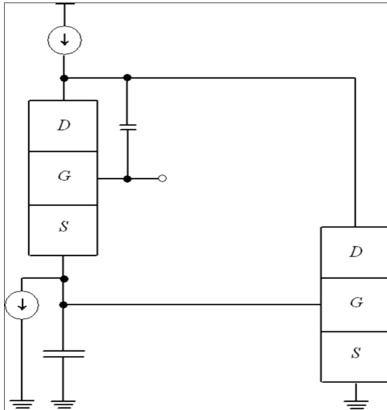
Fig 1a: Structure of the considered filters [19]
