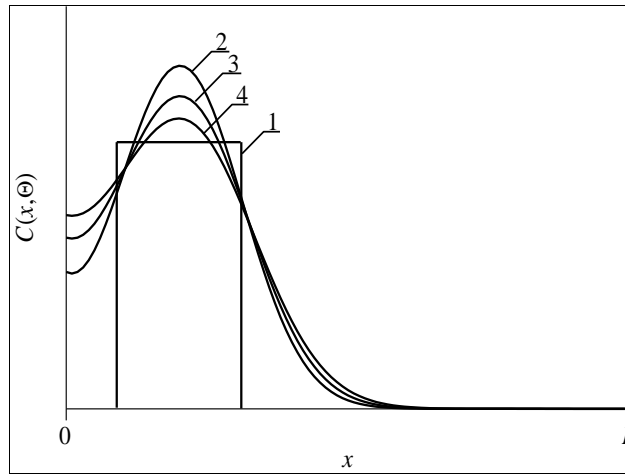
Fig 5: Spatial distributions of dopant in heterostructure after ion implantation. Curve 1 is idealized distribution of dopant. Curves 2-4 are real distributions of dopant for different values of annealing time. Increasing of number of curve corresponds to increasing of annealing time
