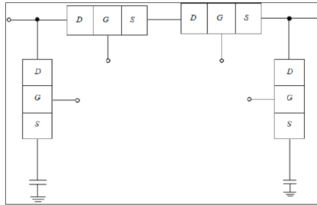
Fig 1a: Structure of the considered circuit of the switch [24]
