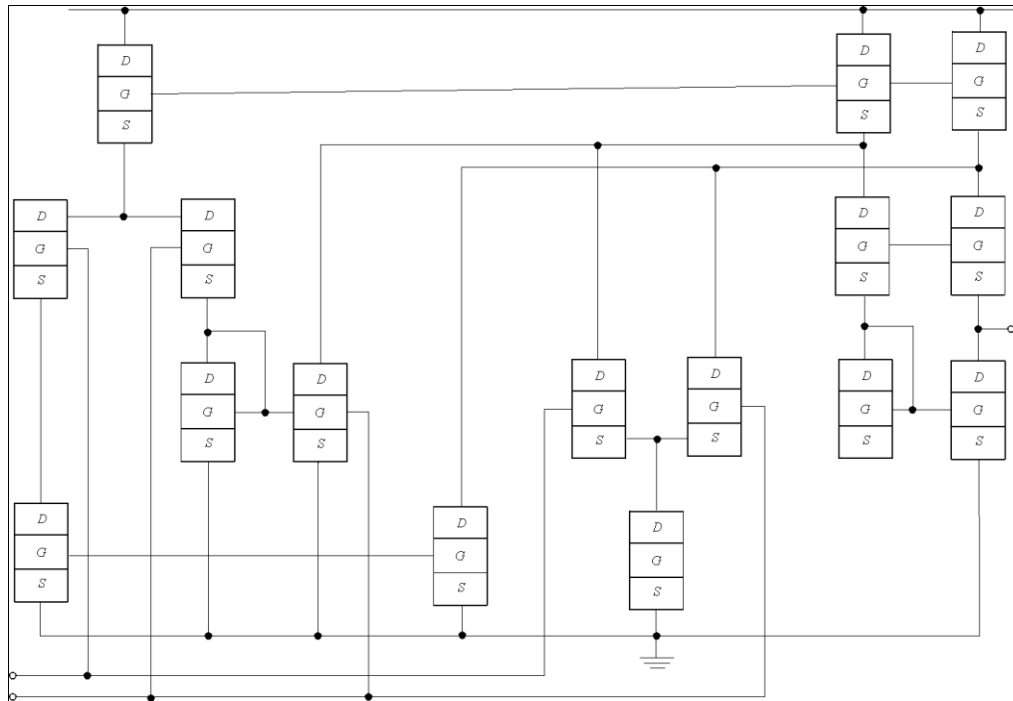
Fig 1a: Structure of the considered amplifier [19]
