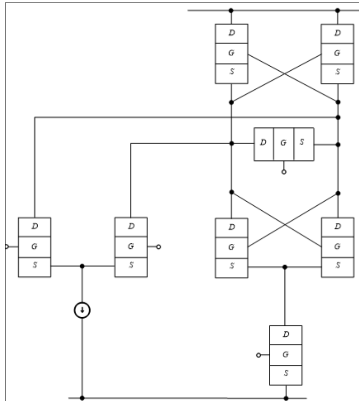
Fig 1: The considered the comparator [4]
