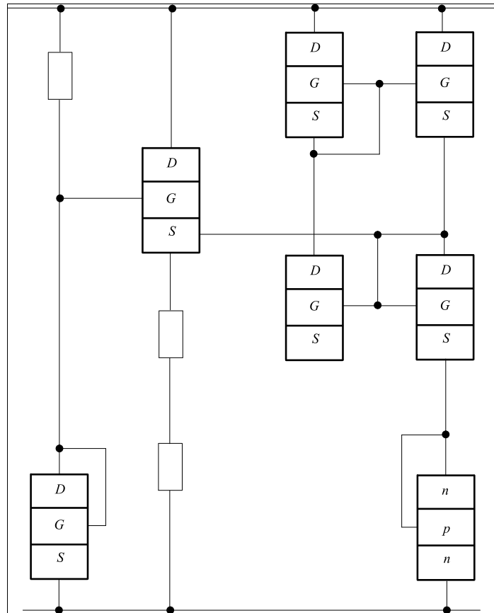
Fig 1a: Structure of the considered amplifier [19]
